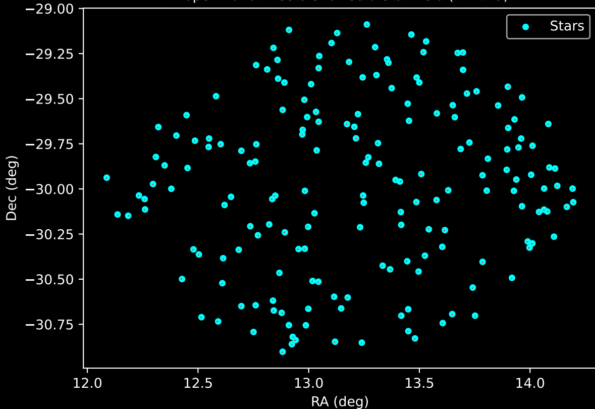
APOGEE DR17 Field: [002-06-O] Proper Motion Vectors for Gaia Star Field (n= 179)
