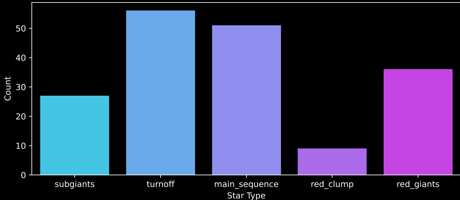
APOGEE DR17 Field: [002-06-O] Count plot of Star Type
