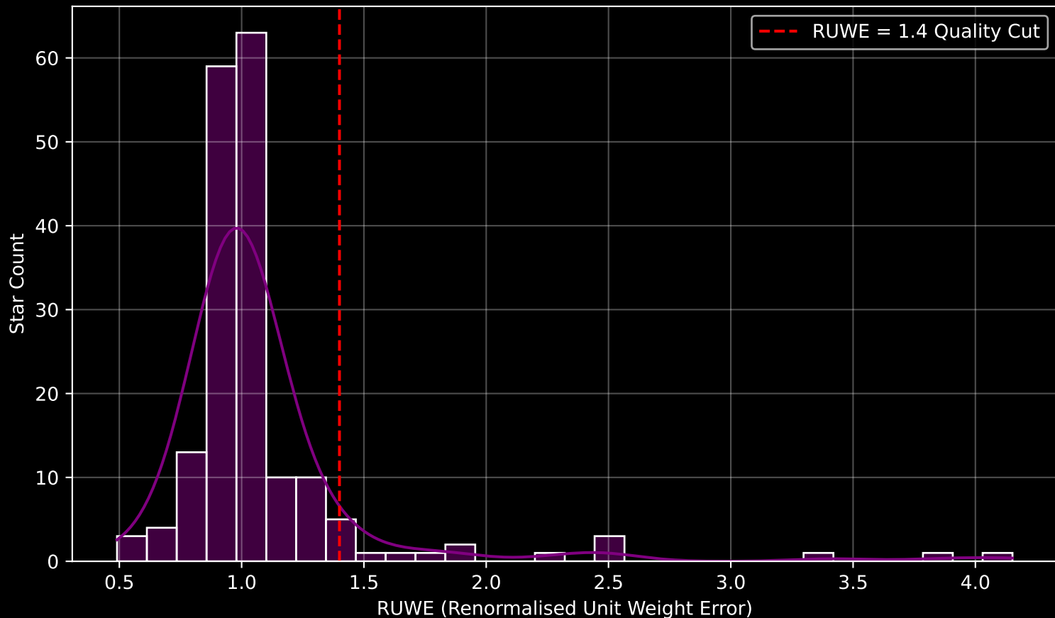
GAPOGEE DR17 Field [002-06-O] RUWE Distribution (n= 179)
