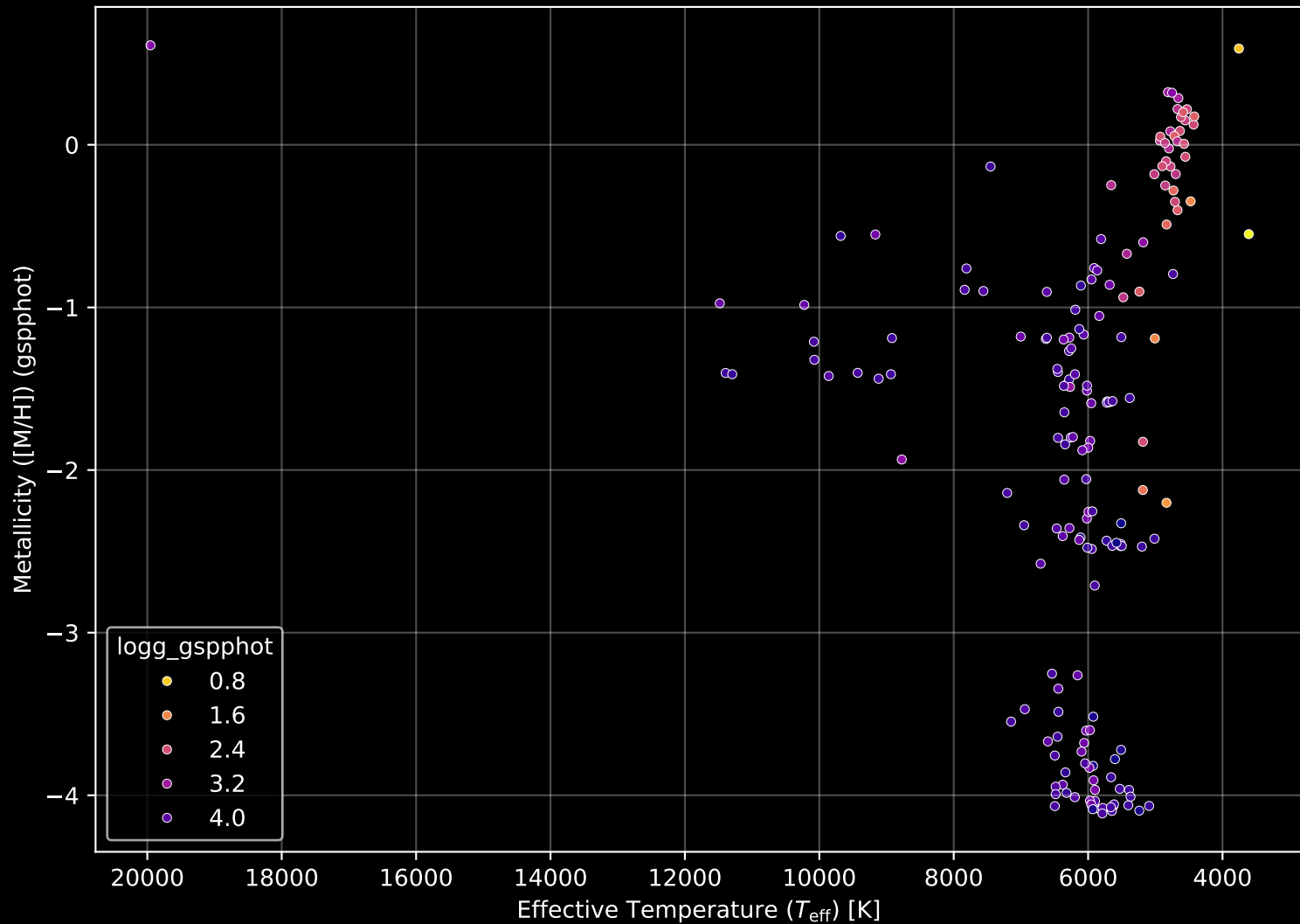
APOGEE DR17 Field: [002-06-O] Stellar Population Parameters (n= 179)
