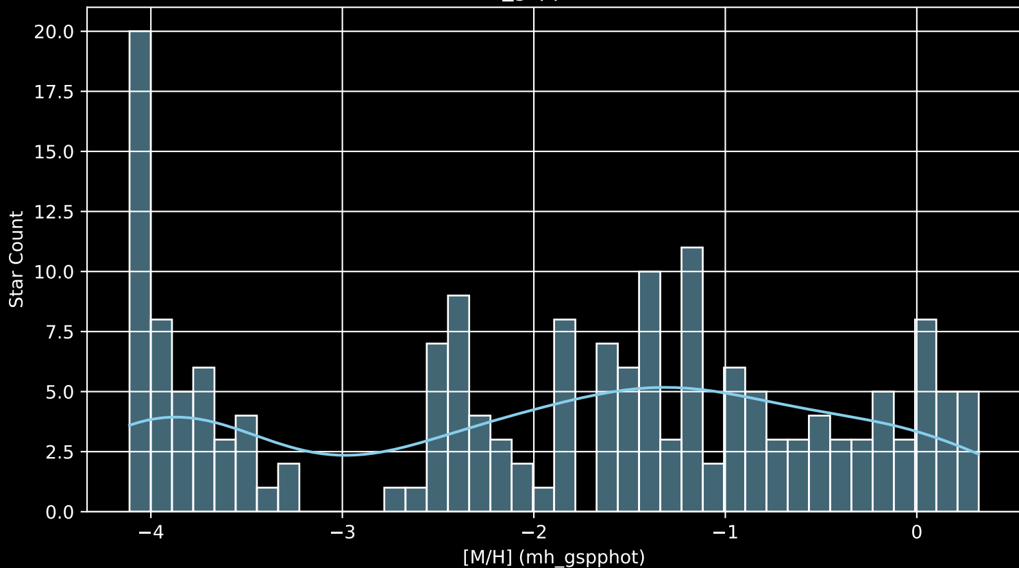
APOGEE DR17 Field: [002-06-O] [M/H] (mh_gspphot) (n= 177)
