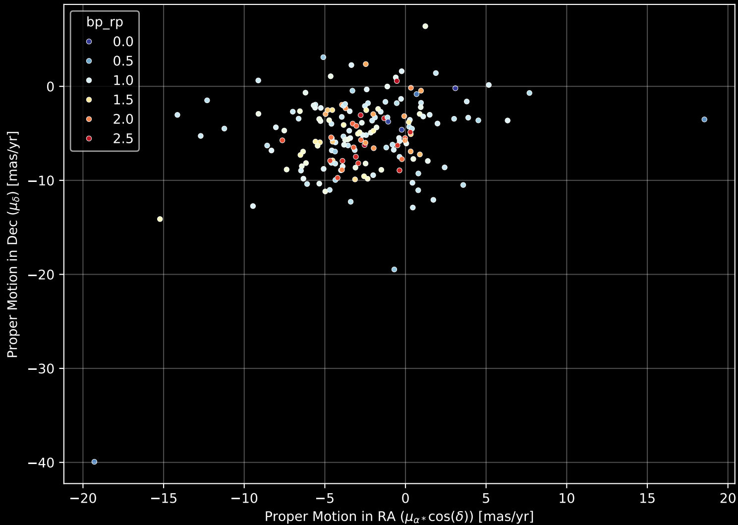
APOGEE DR17 Field: [002-06-O] Proper Motion Diagram (n= 179)
