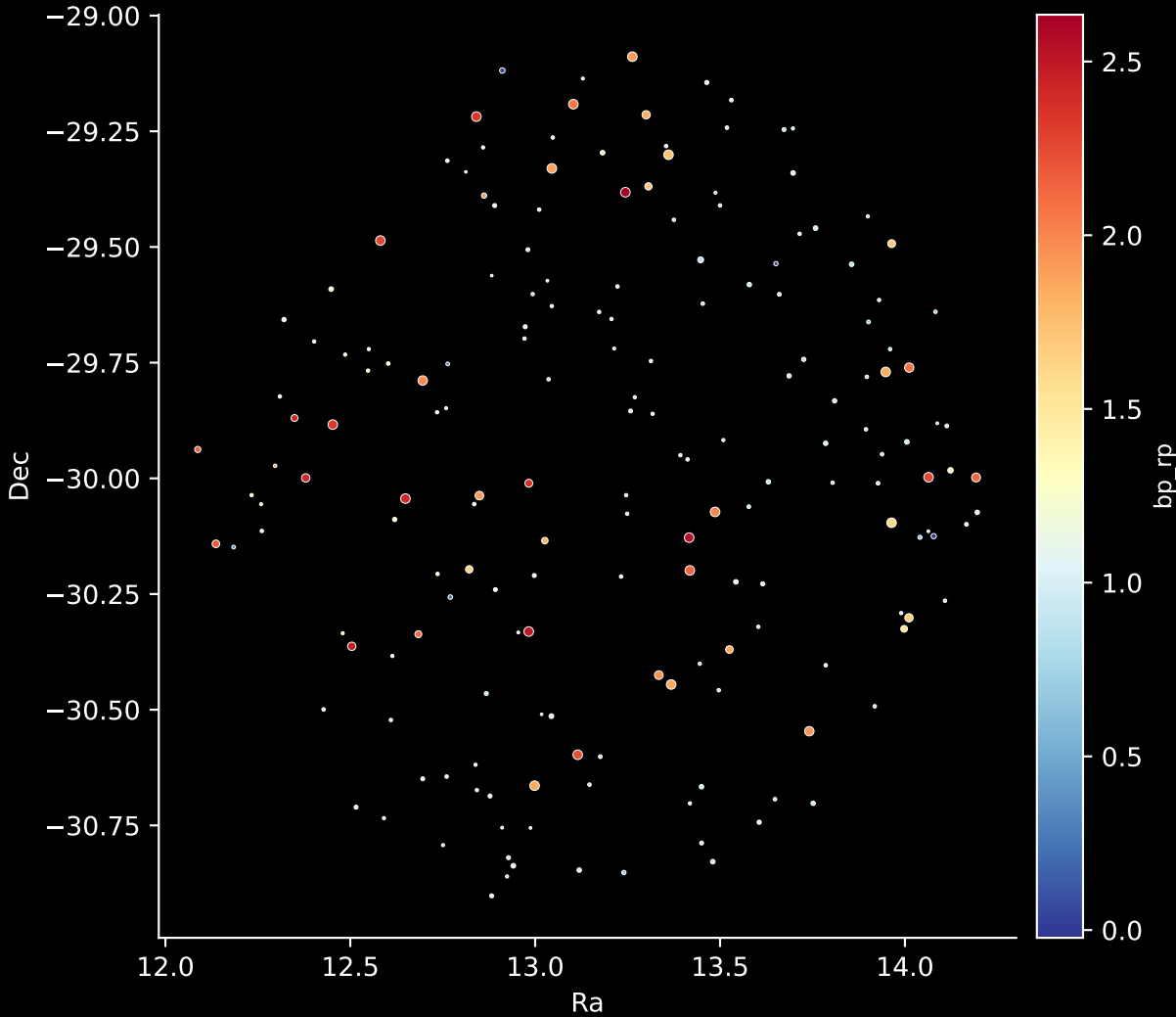
APOGEE DR17 Field: [002-06-O] Stars: 179
