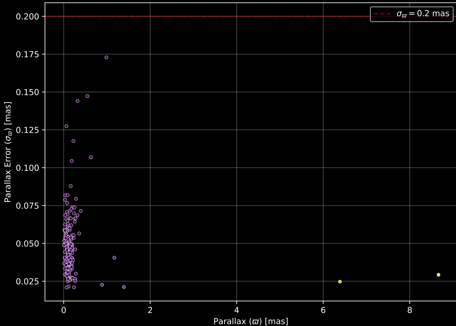
APOGEE DR17 Field: [002-06-O] Parallax Quality (n= 179)
